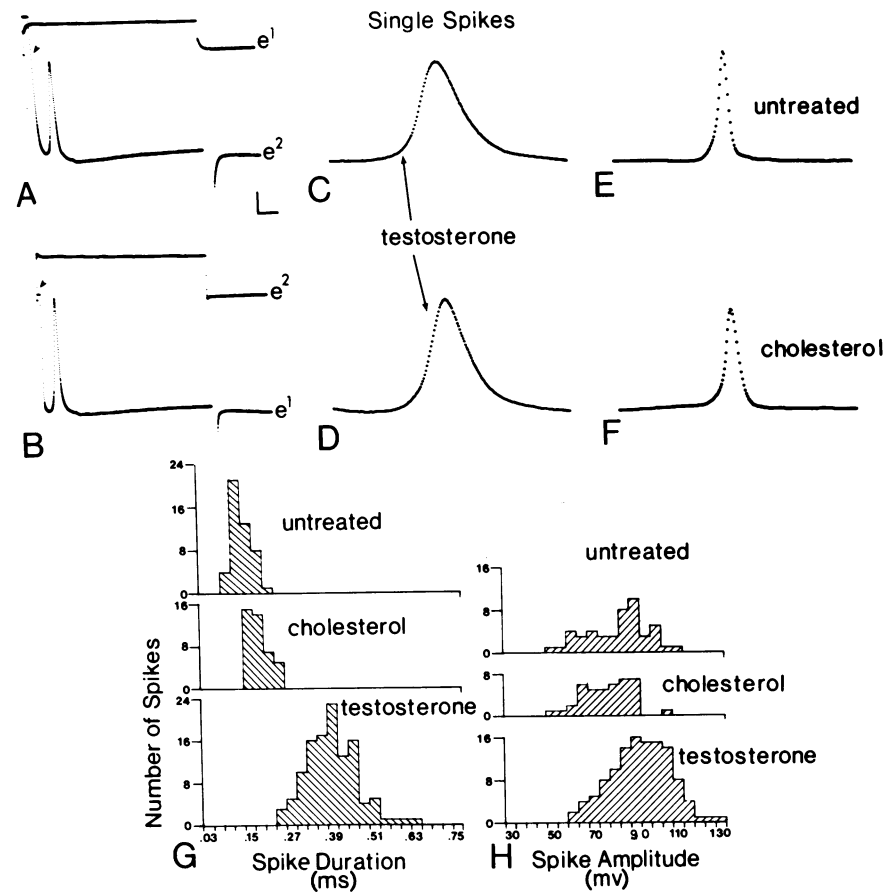
FIG. 2. (A–F) Intracellularly recorded action potentials from single electrocytes. Vertical bar scale in A is 20 mV for all spike records and 1 \mu A for current pulses in top trace of A and B. Horizontal scale is 2.0 msec for A and B and 0.2 msec for C–F. Arrowheads indicate stimulus artifact. (A and B) Each of two electrodes (e 1 , e 2 ) were used alternately for stimulating (square pulses, top trace) and recording so that spikes (bottom traces) were recorded at two positions in a cell. (C–F) The largest class of testosterone-sensitive spikes (as shown on expanded time scale without stimulus pulse) were single spikes. Except where indicated, spike duration or spike amplitude was significantly greater ( P < 0.0001 ) in the testosterone-treated group compared to cholesterol-treated or untreated groups, and these two groups were not significantly different from each other ( P > 0.05 ). Spike duration was 2–3 times greater in testosterone (C and D, which are, respectively, A and B on an expanded scale), compared to untreated (E) or cholesterol-treated (F) groups. (G) Histogram of single spike durations (measured at half-amplitude values). Averages (msec) were as follows: untreated, 0.14 (SD = 0.03; n = 47 ); cholesterol, 0.18 (SD = 0.03; n = 41 ); testosterone, 0.39 (SD = 0.07; n = 113 ). Cholesterol group is significantly greater than untreated one ( P < 0.0001 ). (H) Histogram of total amplitude of single spikes as measured from baseline to peak. Averages (mV) were as follows: untreated, 82.0 (SD = 14.2; n = 47 ); cholesterol, 76.8 (SD = 11.2; n = 41 ); testosterone, 93.4 (SD = 13.7; n = 113 ). Average resting potentials (RPs) or spike thresholds (STs) were not significantly different between any groups: RPs (mV) were as follows: untreated, -92.7 (SD = 6.9; n = 11 ); cholesterol, -95.8 (SD = 9.5; n = 38 ); testosterone, -97.1 (SD = 7.6; n = 83 ). STs ( \mu A) were as follows: untreated, 0.9 (SD = 0.5; n = 45 ); cholesterol, 1.0 (SD = 0.4; n = 50 ); testosterone, 1.0 (SD = 0.5; n = 122 ).
