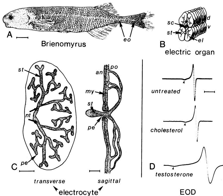
FIG. 1. (A) Line drawing of Brienyomys indicating position of electric organ (eo). (Bar = 1 cm.) (B) Oblique anterior view of electric organ, which consists of two dorsal (d) and two ventral (v) columns of serially stacked cells called electrocytes (el). Each electrocyte is separated within a gelatinous compartment from its neighbor. The columns surround the spinal cord (sc), which contains the electromotoneurons that synchronously activate all of the electrocytes. (C) Line drawings of electrocytes. To the left is a transverse view looking at the anterior face of the electrocyte labeled el in B. The stalk system (st, also in B) has several branches but is innervated by electromotoneurons in a restricted zone (nt). To the right is a sagittal view showing the anterior (an) and posterior (po) faces of the electrocyte. A stalk branch penetrates through the electrocyte body at a particular site (pe, also see transverse view) and has small branches that are continuous with the posterior face. A central zone of myofilaments (my) denotes the electrocytes' origin from striated muscle. [Bars = 500 (transverse) \mu\text{m} and 30 (sagittal) \mu\text{m} .] (D) Differential recordings (positive electrode near the head) of the EOD of Brienyomys sp. scaled to the same peak-to-peak amplitude. Shown are representative EODs of untreated, cholesterol-treated (18 days), and testosterone-treated (18 days) individuals. Arrowheads indicate small initial negative phase of the EOD. (Bar = 0.4 msec.) Average EOD durations (msec) were as follows: untreated, 0.6 (SD = 0.05; n = 12); cholesterol-treated, 0.7 (SD = 0.05; n = 3); testosterone-treated, 1.9 (SD = 0.44; n = 9).
