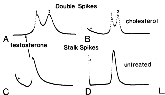
FIG. 3. (A–D) Additional classes of testosterone-sensitive spikes: double and stalk spikes. Action potentials recorded intracellularly from single electrocytes as in Fig. 2. Vertical bar scale in A is 20 mV for all records. Horizontal scale is 0.2 msec for A and B and 0.5 msec for C and D. Duration measurements as in Fig. 2. Double spikes: total (spikes 1 and 2 combined) duration in testosterone-treated specimens (A) was 2–3 times greater than cholesterol-treated (B) or untreated ones. Averages (msec) were as follows: testosterone, 0.78 (SD = 0.22; n = 12 ); cholesterol, 0.32 (SD = 0.09; n = 6 ); untreated, 0.28 (SD = 0.07; n = 4 ). Average duration (msec) of spike 1: testosterone, 0.27 (SD = 0.06; n = 7 ); cholesterol, 0.13 (SD = 0.01; n = 2 ); untreated, 0.10 (SD = 0.06; n = 2 ); spike 2: testosterone, 0.36 (SD = 0.11; n = 9 ); cholesterol, 0.15 (SD = 0.04; n = 2 ); untreated, 0.15 (SD = 0.03; n = 2 ). There were no significant differences ( P > 0.1 ) between spikes 1 and 2 within any experimental group. Some spikes could not be measured because their falling or rising phase did not extend below half-amplitude values because of overlap of the two spikes. Stalk spikes: spike duration in the testosterone treatment group (C) was significantly greater than cholesterol ( P < 0.005 ) or untreated (D) ( P < 0.01 ) ones. Averages (msec) were as follows: testosterone, 0.62 (SD = 0.2; n = 8 ); cholesterol, 0.38 (SD = 0.05; n = 4 ); untreated, 0.33 (SD = 0.07; n = 4 ). The small number of cases in which we recorded stalk spikes most likely results from the lower probability of impaling a stalk branch, which is a thin cable-like structure (see Fig. 1C). In 9 of 13 cases, recordings of double spikes on one electrode coincided with recording a stalk spike on a second electrode. This is expected when the stalk electrode is used for stimulation, which might initiate a sequential activation of the two faces and so double spikes (6).
